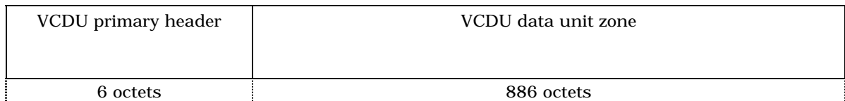
Figure 8-2 VCDU structure
